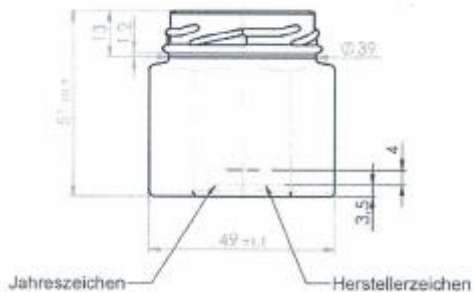
43mm RTO FLAT FD-157
